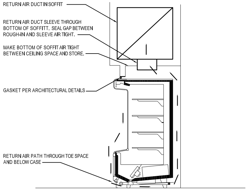
TYPICAL UNDER CASE RETURN AIR DETAIL AT WALL
